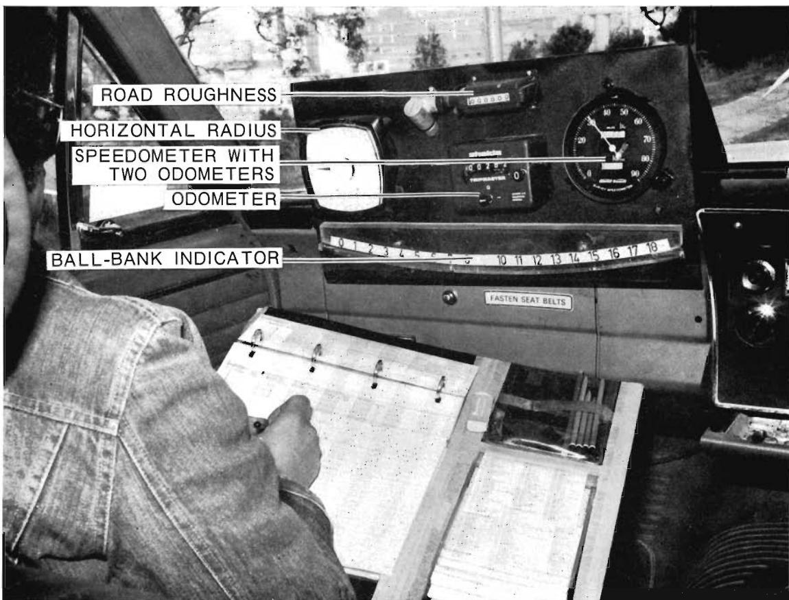
Plate 6—Road inventory vehicle—instrument panel and recording position.
