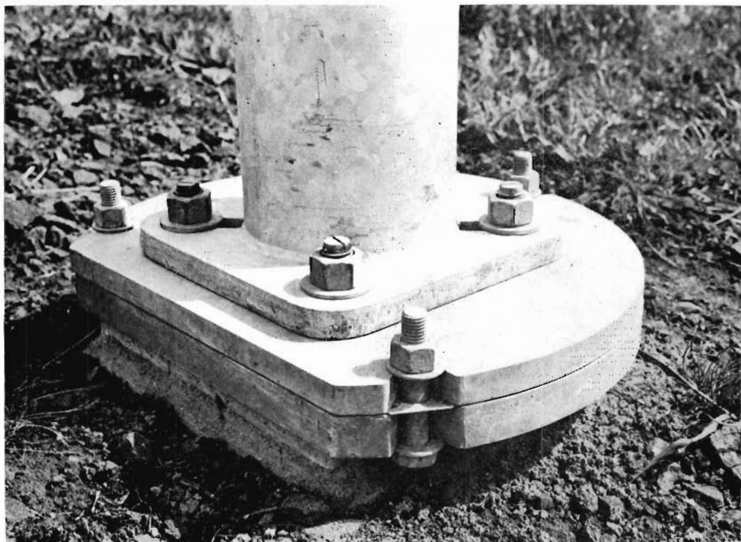
Plate 13—A slip base assembly. In the foreground can be seen the V-notches in the top and bottom slip base plates, the keeper sheet between the plates, and one of the bolts that hold the plates and sheets together.
