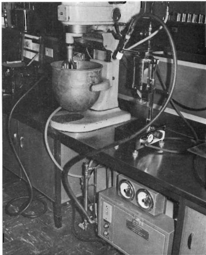
Plate 17—Laboratory apparatus for production of foamed bitumen for testing purposes. A measured quantity of bitumen is held in the cylinder at the top right of the photograph. Compressed air is used to force the bitumen up into the nozzle to the left of the cylinder. Steam from the generator below the bench passes through the same nozzle and causes the bitumen to foam or expand. The foamed bitumen is mixed with soil in the bowl beneath the mixer.
