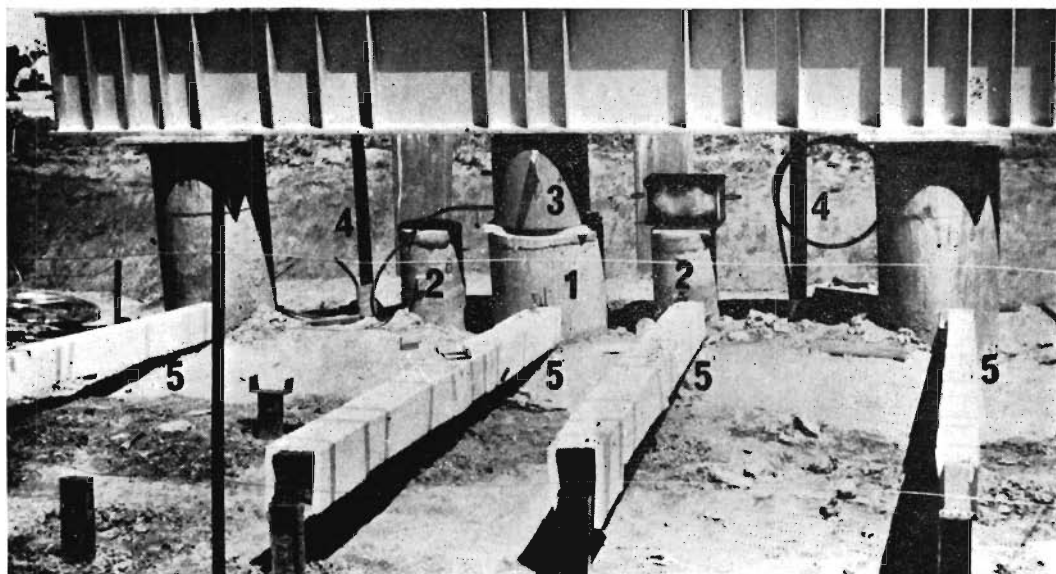
Plate 16—Gladstone Road pile loading study.
