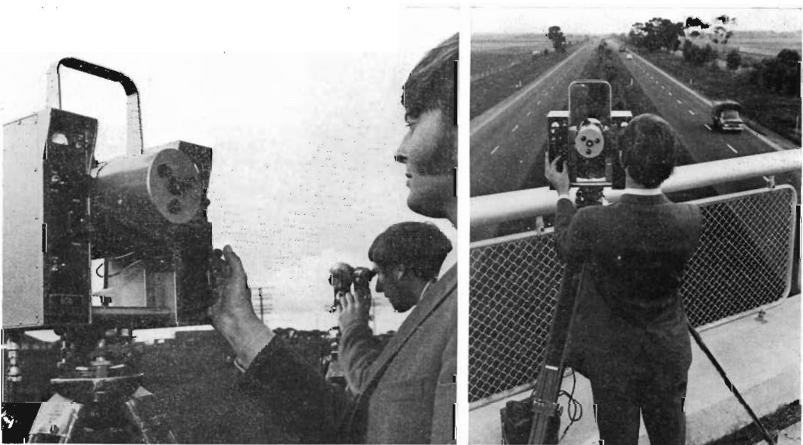
Plates 8 and 9—Use of the Board's Geodimeter 6A electronic distance measuring equipment during a project control survey.
