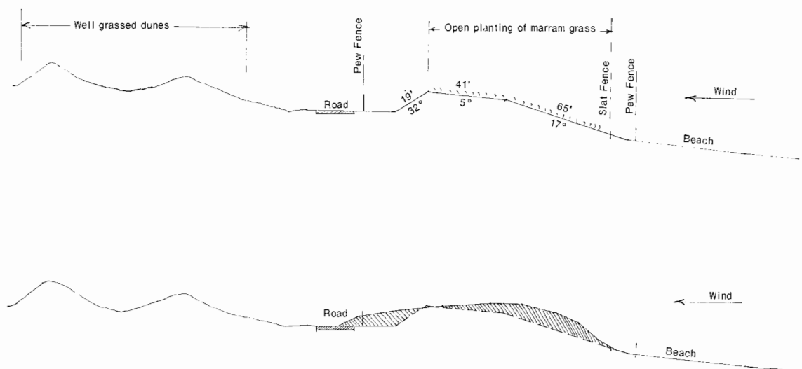
Figure 9— Top: designed profile of "Dune 42". Bottom: profile towards which the dune tends to revert. Regular maintenance is needed to counteract this tendency.
