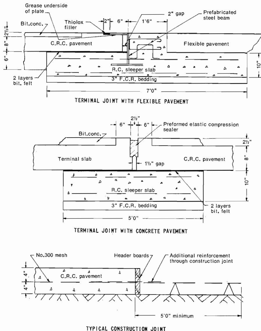
Figure 6—C.R.C. pavement. Details of terminal joints and a construction joint.
