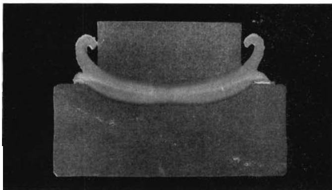
Plate 12—Cross section of a \frac{3}{4} in. friction welded stud, x 2.
