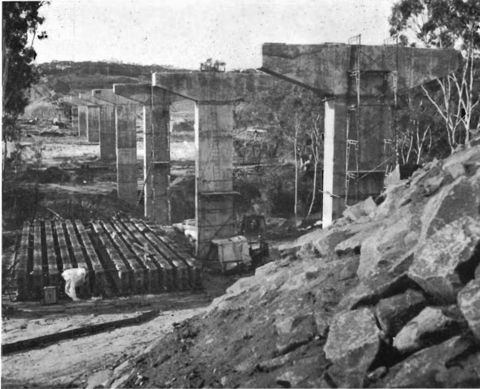
Plate 9 — Construction of the Glenelg River Bridge, Princes Highway West, Dartmoor.
