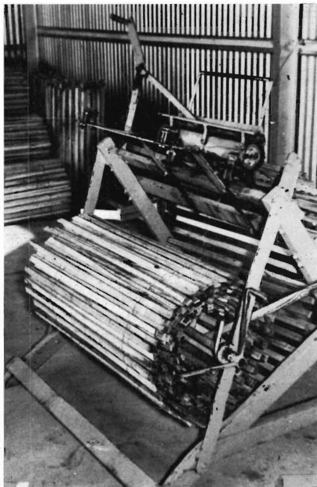
Plate 4 — Sand Drift Control. Machine Designed by Soil Conservation Authority for Production of Slat Fencing.
