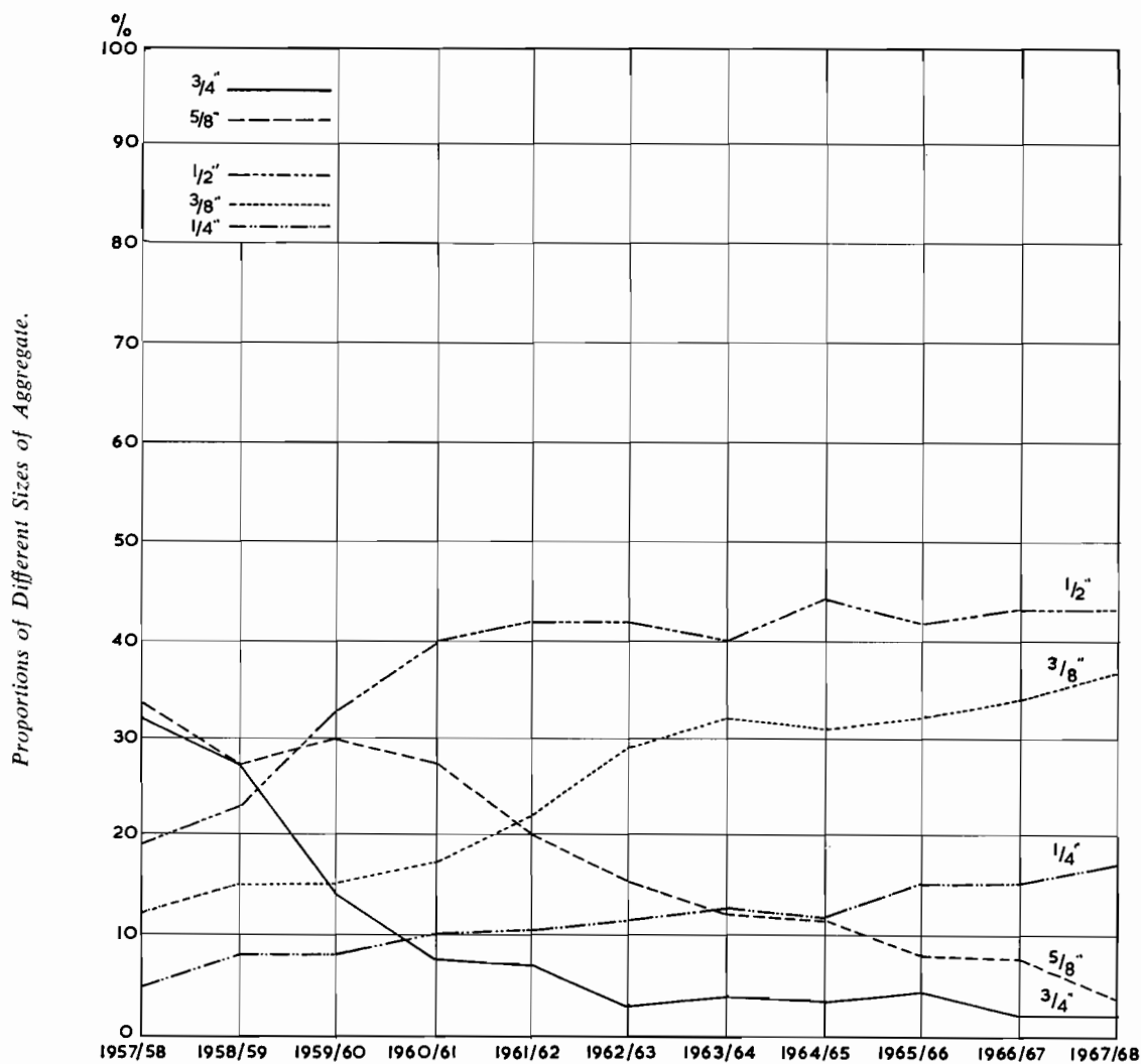
Figure 2 — Change in Usage of Different Sizes of Aggregate, 1957/58–1967/68.
