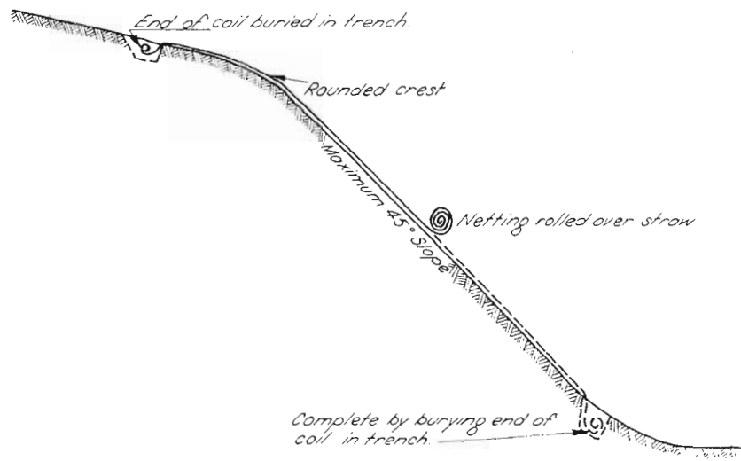
Figure 1 — Batter Stabilisation. Cross Section showing Method of Securing Straw with Wire Mesh.
