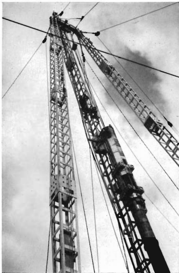
Plate 2—Maribyrnong River Bridge, Raleigh's Road. Pile driving in progress.
