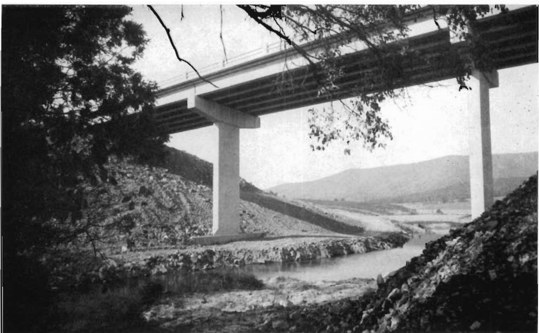
Three span reinforced concrete bridge over Sandy Creek on the Nillahcootie deviation.
